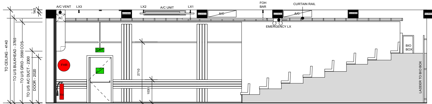
PROMPT SIDE ELEVATION PLEASE CHECK DIMENSIONS IN THEATRE
